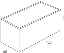
RECTANGULAR PLANTER 60x120x60 cm
