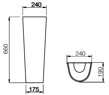
Cento Colonna Pedestal Pedestal COD. 40009
