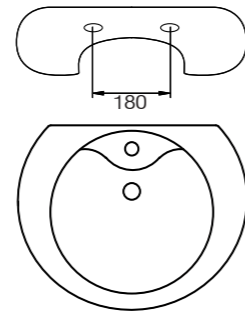
Cento Lavabo cm62 Washbasin cm62 Lavabo cm62 COD. 40005
