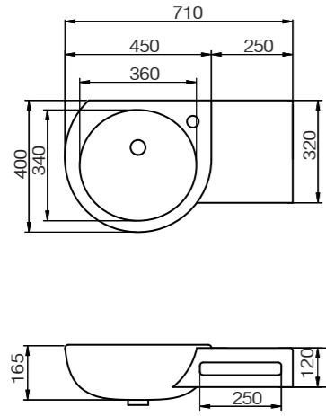
Cento Lavabo DX Washbasin DX Lavabo DX COD. 40007
